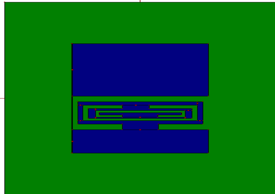
Fig 2: Proposed Rectangular Micro-strip Patch Antenna with C inside C Shaped Slots Feed at (-5, -8)Point
