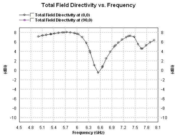
Fig 8: Total field directivity & frequency of Rectangular Micro-strip Patch Antenna with C insideC shaped slots
