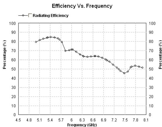
Fig 11: Radiating efficiency & frequency of Rectangular Micro-strip Patch Antenna with C inside C shaped slots
