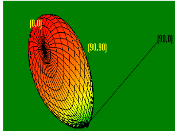
Fig 12: 3D radiation pattern for 6 GHz frequency of Rectangular Micro-strip Patch Antenna with C inside C shaped slots
