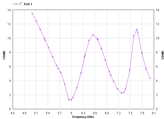
Fig 3: VSWR of the Proposed Rectangular Microstrip Patch Antenna with C inside C shaped slots
