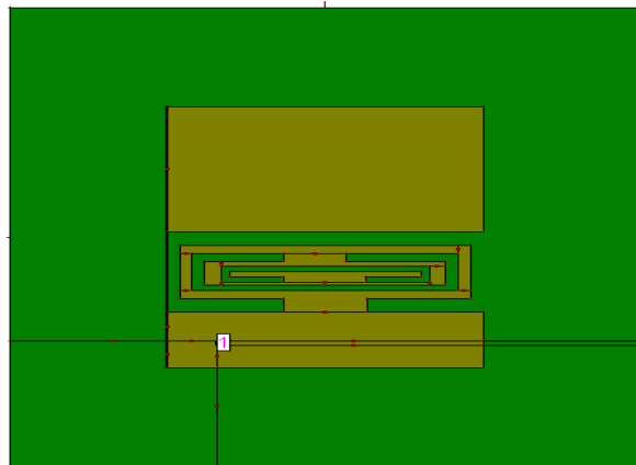
Fig 2: Proposed Rectangular Micro-strip Patch Antenna with C inside C Shaped Slots Feed at (-5, -8)Point
