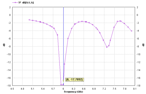
Fig 7: Total field gain & frequency of Rectangular Micro-strip Patch Antenna with C inside C shaped slots
